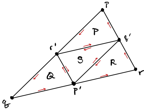
FIGURE 6.4. The midpoint subdivision of T . We label the vertices of all of the triangles. We also decorate the edges of the four smaller triangles with their orientations.
